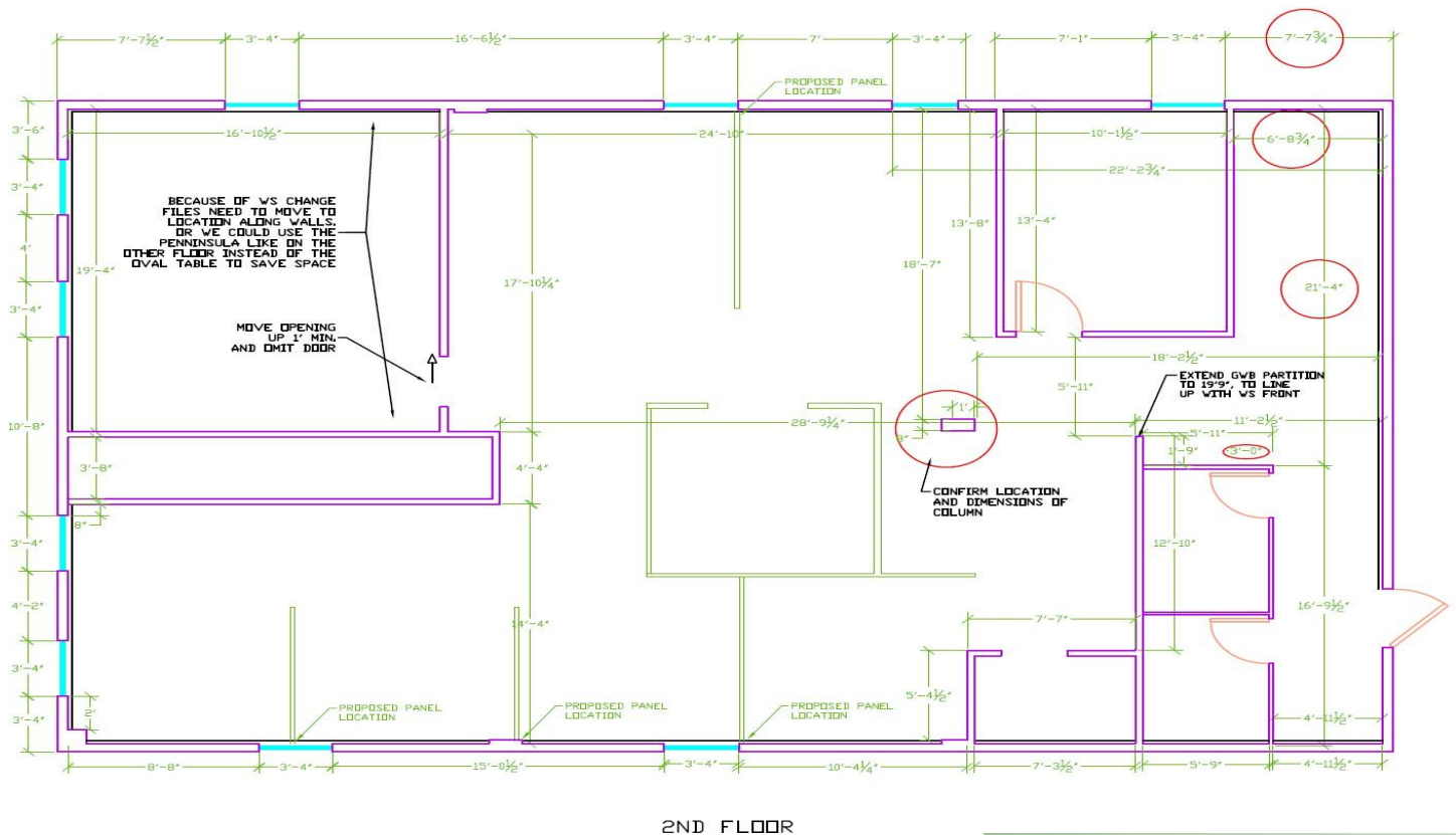
2ND FLOOR
